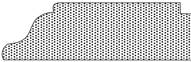
BLBM001 9/16" x 2"
