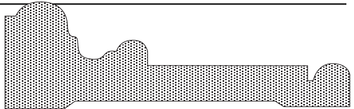
BLCS092 1-1/8" x 3-1/2"
