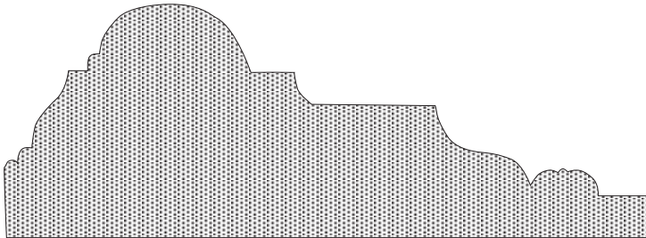
BLCHR136 1-1/8" x 3-1/8"
